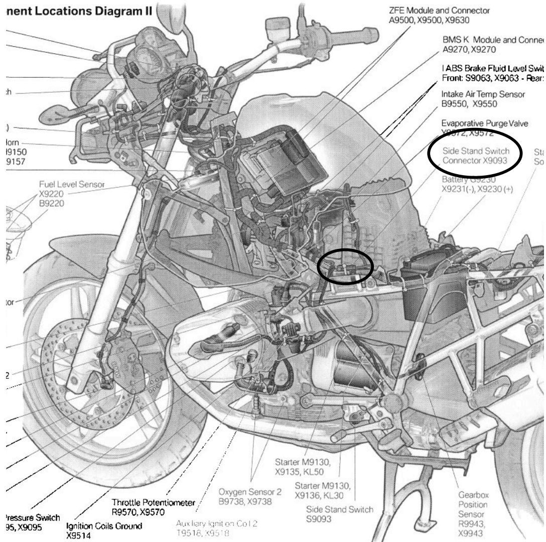
Figure 1: Location of Connector X9093 (R1200GS)
