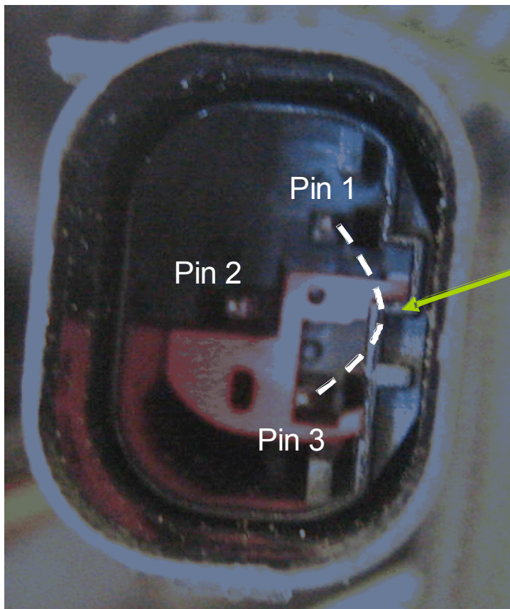
Chassis side of connector X9093 Showing Which Pins/Wires to Connect (Note male pins and connector orientation)
