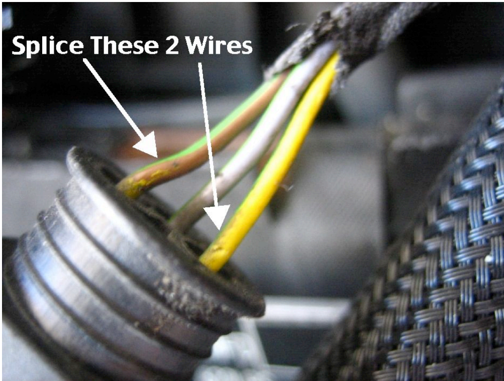
Rear of Connector X9093 (Chassis Side) Showing the Wires that Need to be Spliced
