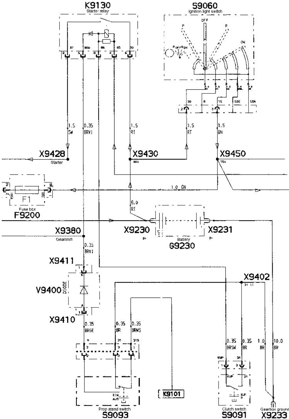
Figure 3: R1150 Side-Stand Safety Interlock Schematic
