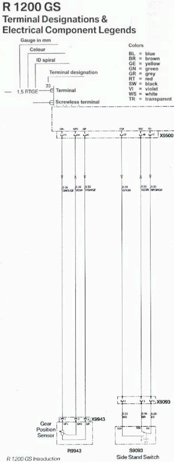
Figure 2: R1200 Side-Stand Safety Interlock Schematic
