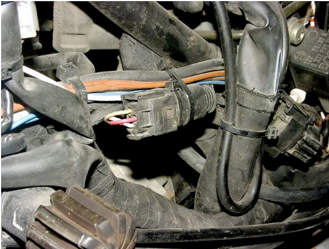
Location of Connector X9093 on R1150GS: Shot 1
