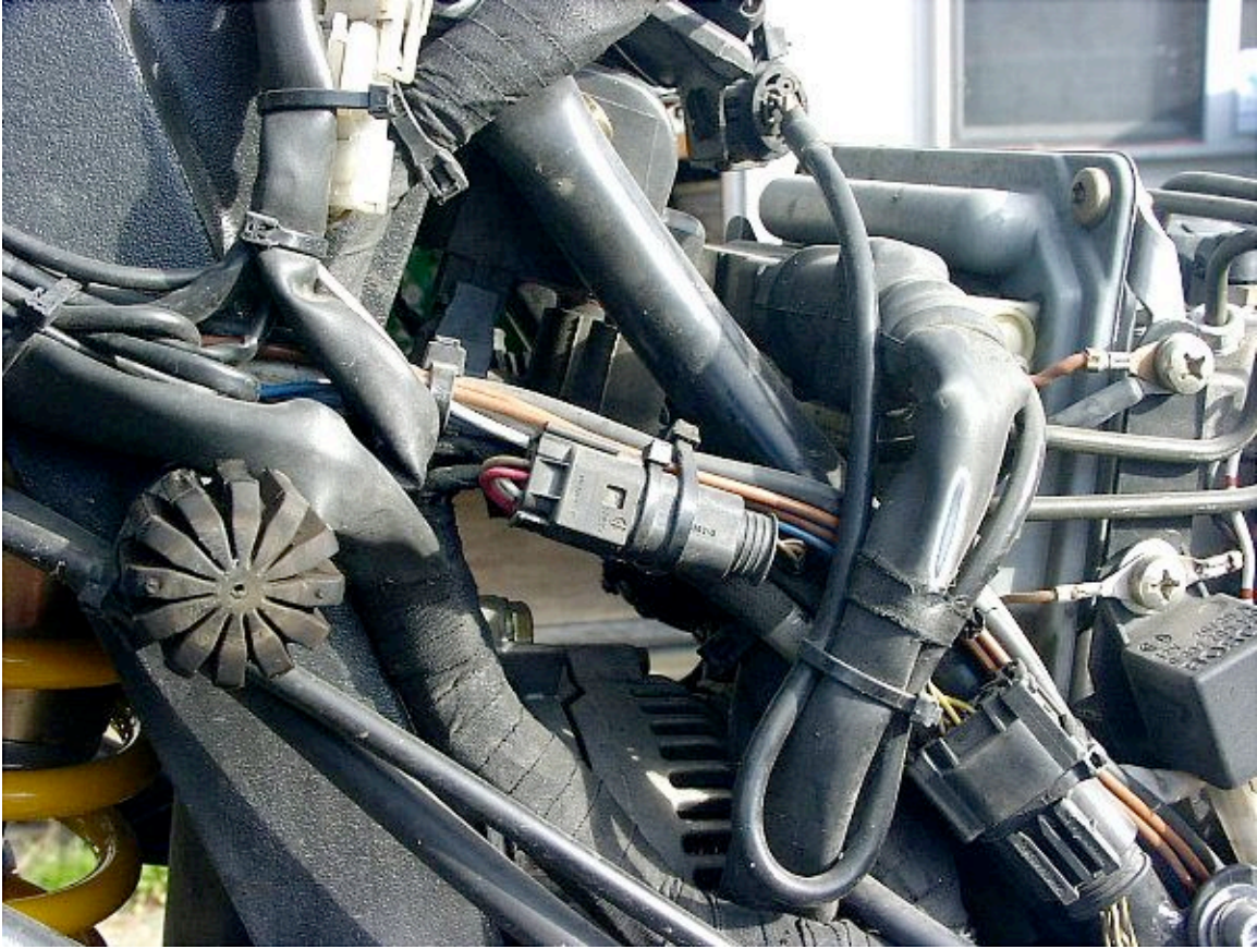
Location of Connector X9093 on R1150GS: Shot 2
