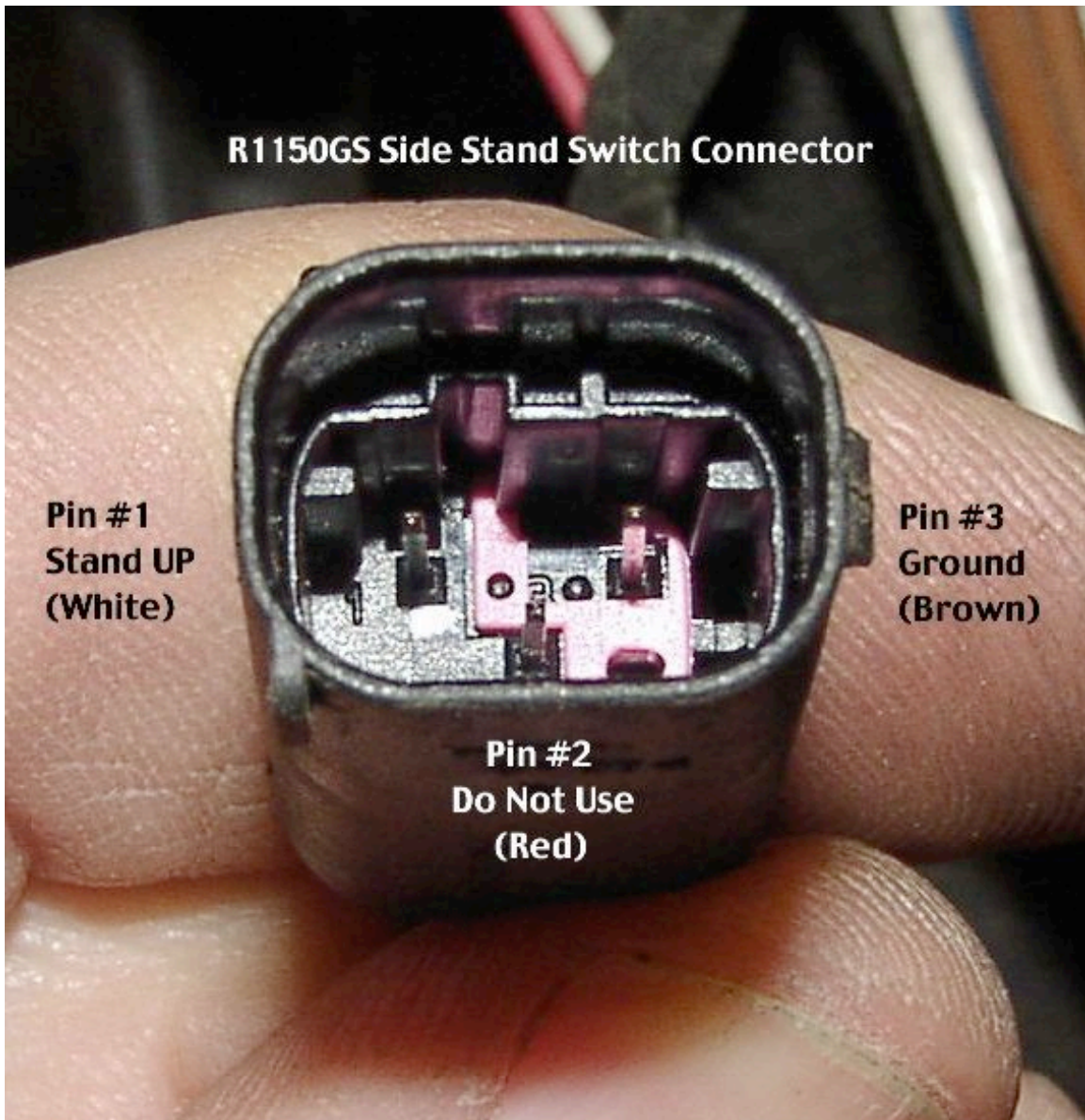
Close-up of Connector X9093 on R1150GS
